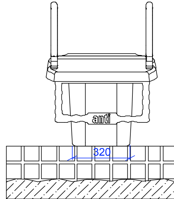
Pool Elevation
